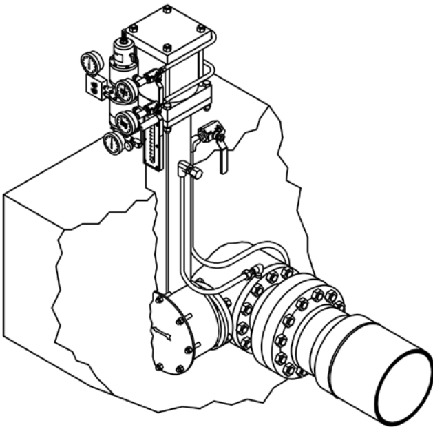
Figure 3 – Below Ground Regulator Design Permits Easy Maintenance
