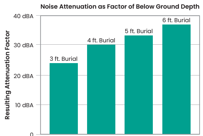
Figure 5 – Noise Attenuation as Factor of Depth
